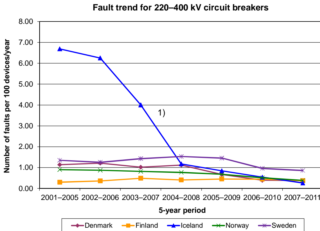
FIGURE 5.11 FAULT TREND FOR CIRCUIT BREAKERS AT VOLTAGE LEVEL 220–400 kV.
