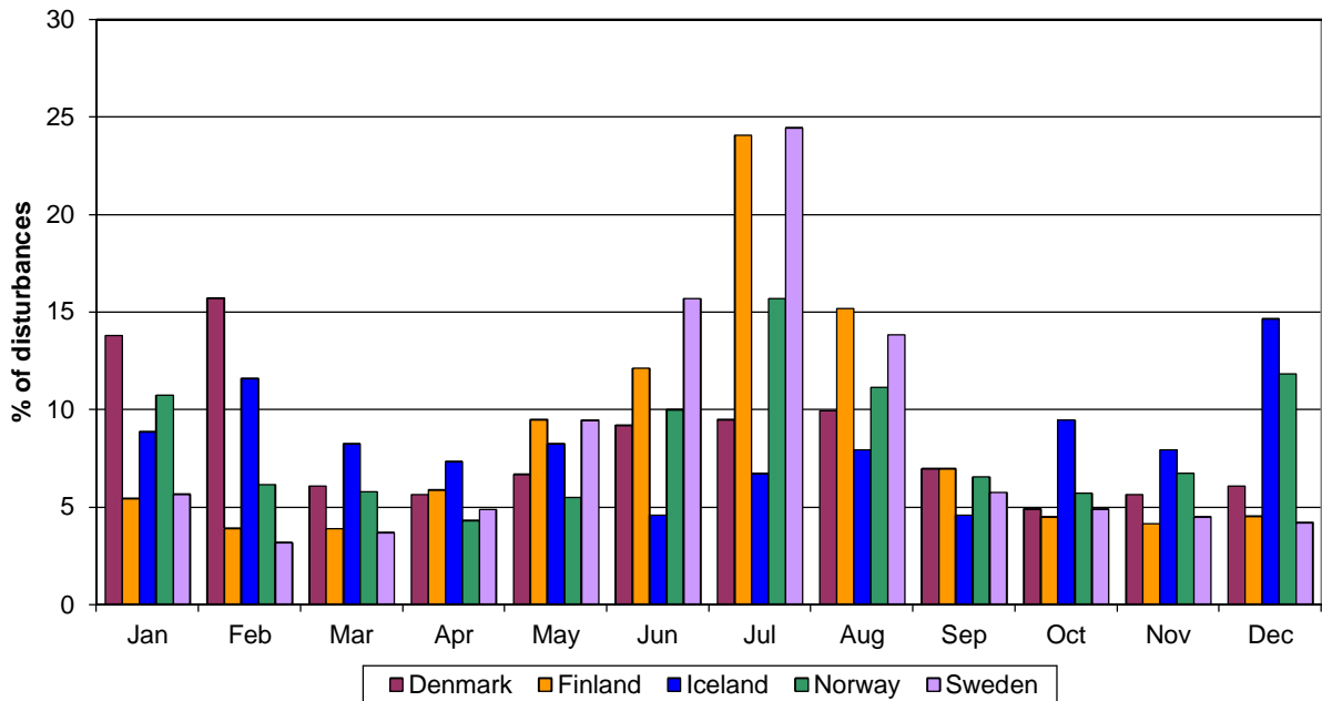
FIGURE 3.3 AVERAGE PERCENTAGE DISTRIBUTION OF GRID DISTURBANCES ACCORDING TO MONTH FOR THE PERIOD 2002–2011.
