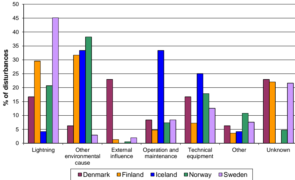
FIGURE 3.4 PERCENTAGE DISTRIBUTION OF GRID DISTURBANCES ACCORDING TO CAUSE IN 2011.
