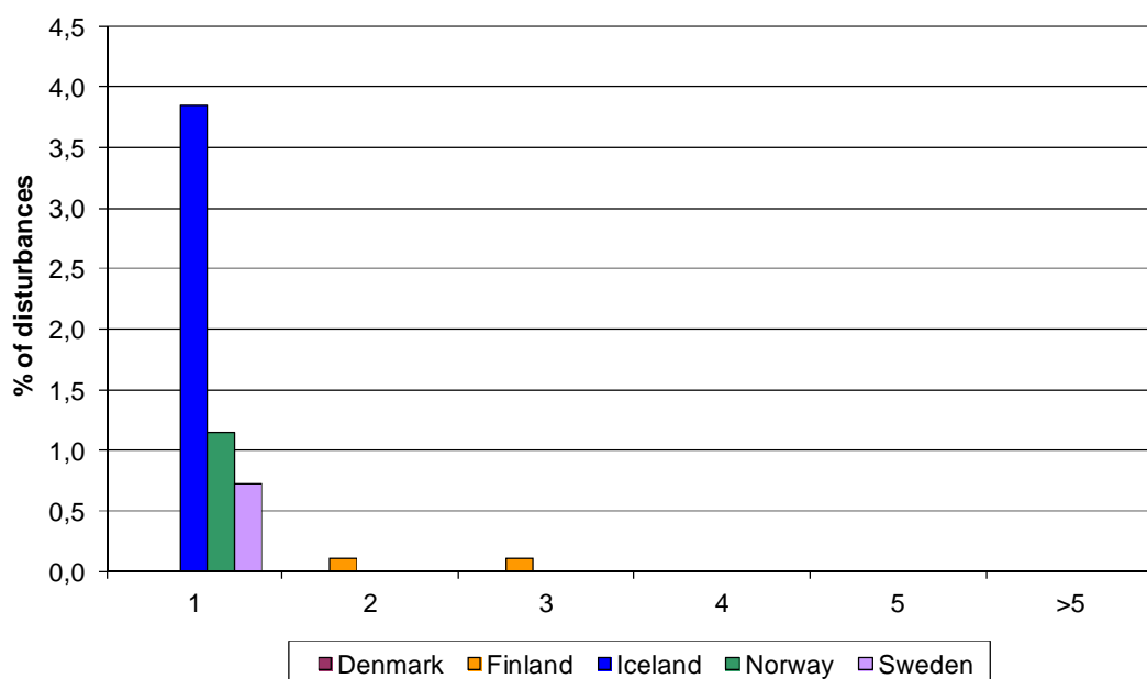
FIGURE 6.3 GROUPING OF BUSBARS ACCORDING TO NUMBER OF OUTAGES IN 2011.
