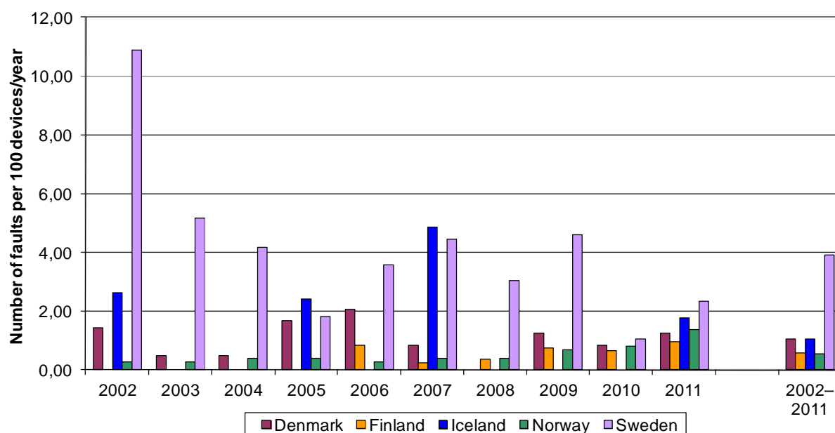
FIGURE 5.6 ANNUAL DIVISION OF FAULTS DURING THE PERIOD 2002–2011.
