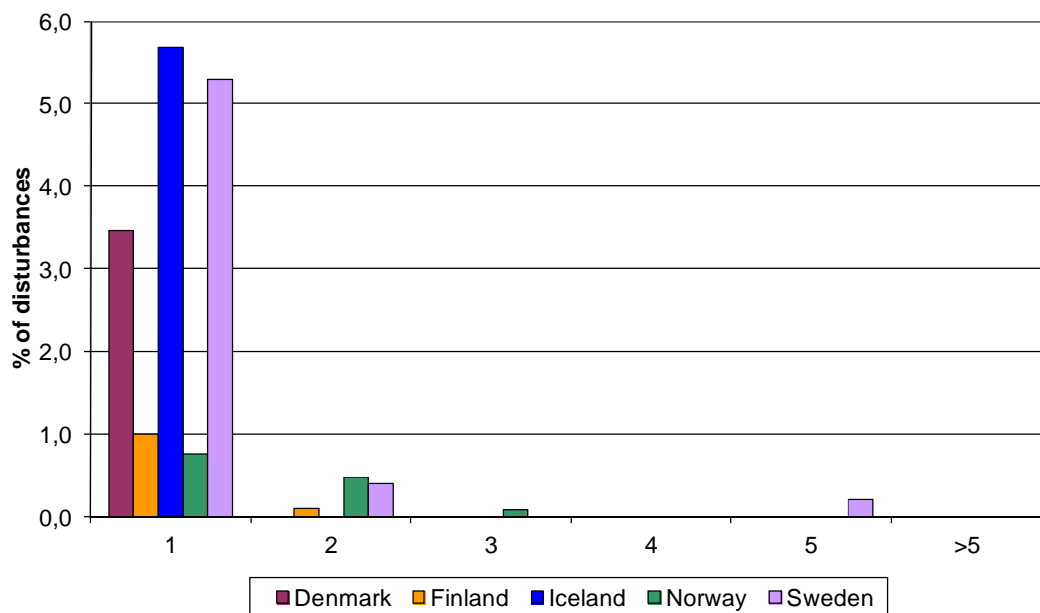
FIGURE 6.2 GROUPING OF TRANSFORMERS ACCORDING TO NUMBER OF OUTAGES IN 2011.
