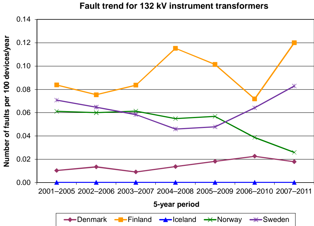
FIGURE 5.10 FAULT TREND FOR INSTRUMENT TRANSFORMERS AT VOLTAGE LEVEL 132 kV.
