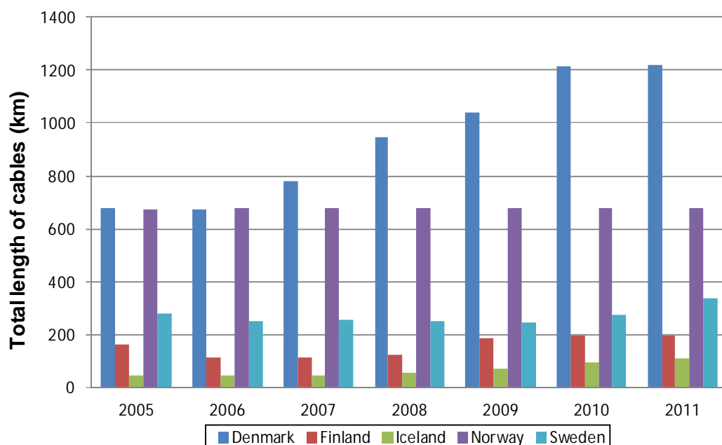
FIGURE 5.6 TOTAL LENGTH OF CABLES AT ALL VOLTAGE LEVELS DURING THE PERIOD 2005-2011.
