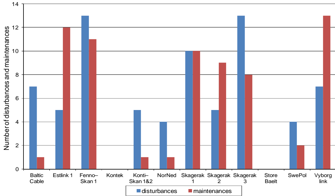
FIGURE 7.6 ALL HVDC DISTURBANCES AND MAINTENANCES IN 2011
