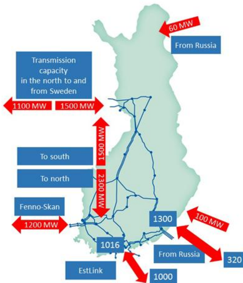
Figure 1. Commercial maximum transmission capacities in the Finnish transmission grid in 2015.
