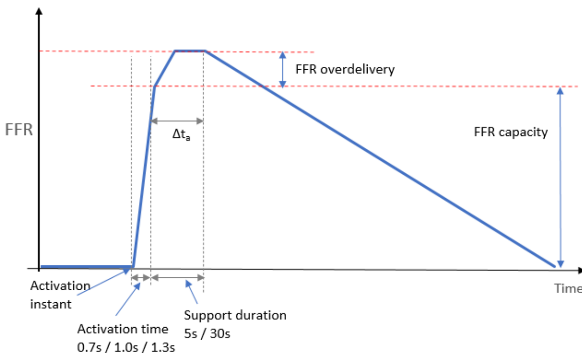
Figure 3.1 Activation of Fast Frequency Reserve
